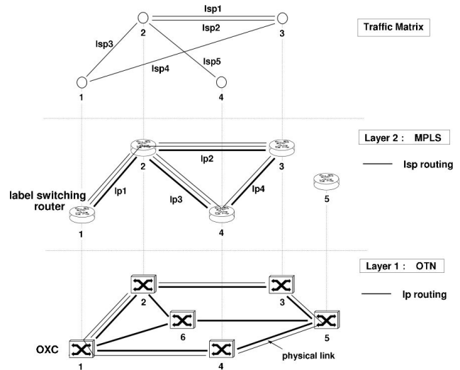
Fig. 1. Architecture of the MPLS over OTN.
